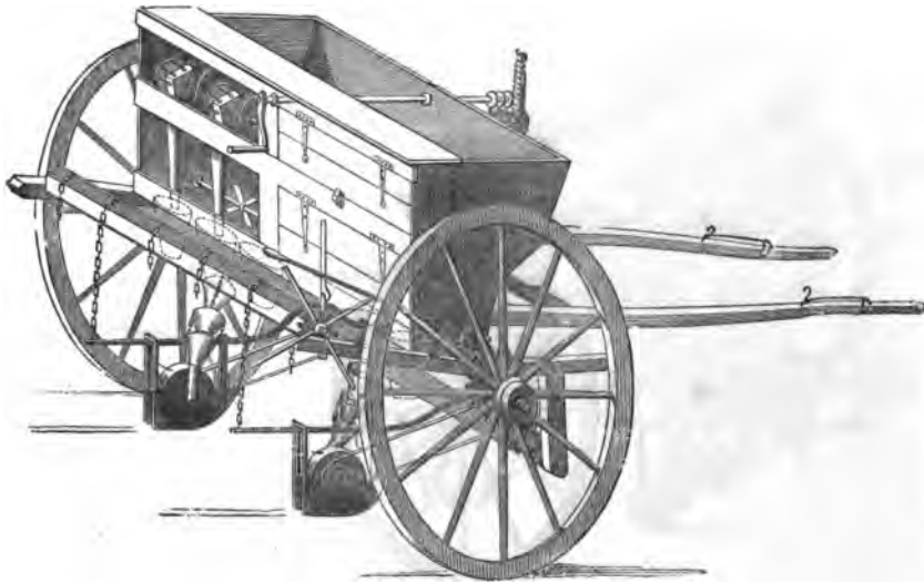
HORNSBY'S PATENT DROP DRILL.
